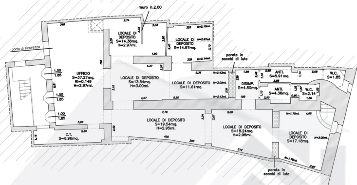
PIANO TERRA
