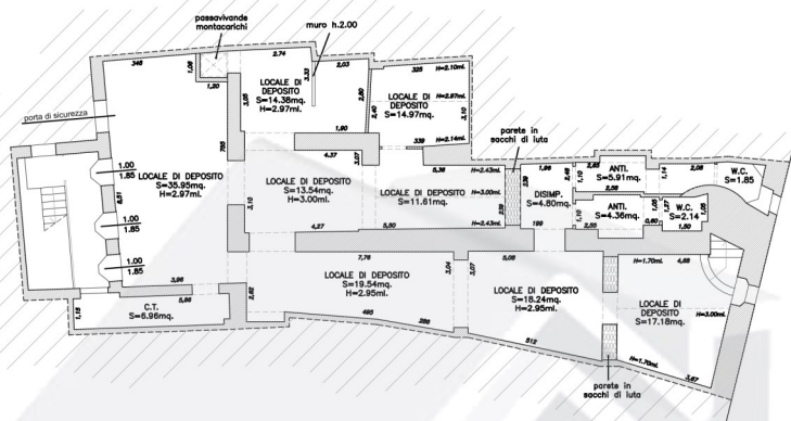
PIANO TERRA
